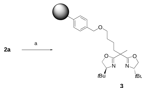
Scheme 2. a) Styrene, DVB ( 2a :styrene:DVB = 7:42:51), AIBN, toluene (60% v/v), 80 °C, 18 h. AIBN = azobisisobutyronitrile.
